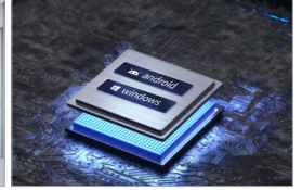
Android 11.0 system
